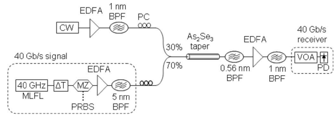
Fig. 4. Experimental setup for 40-Gb/s wavelength conversion in a 16-cm length tapered \text{As}_2\text{Se}_3 fiber.
