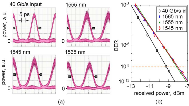
Fig. 9. (a) 40-Gb/s signal eye diagrams at converted and original wavelengths from 22.5-cm length \text{As}_2\text{S}_3 rib waveguide. (b) BER performance of wavelength-converted 40 Gb/s signals.
